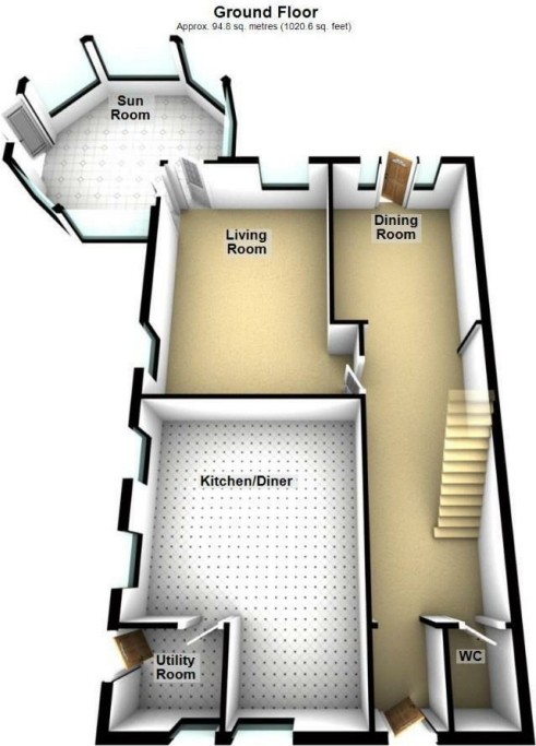
Total area: approx. 172.2 sq. metres (1853.2 sq. feet) Please be advised the floorplans are not drawn to scale and are to be used to give an idea of the layout of the property. Plan produced using PlanUp.
